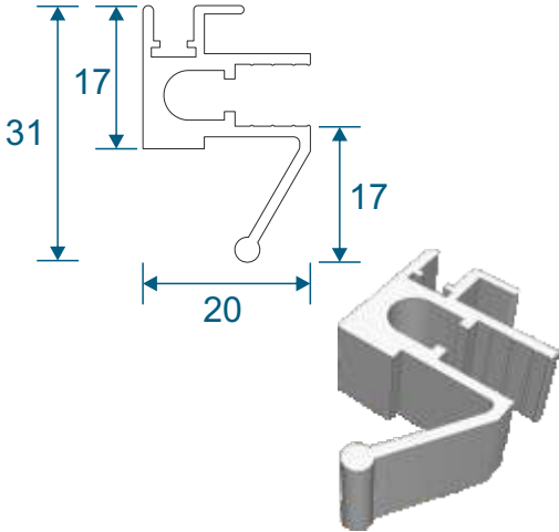
SG87 - Outer Frame Bottom
